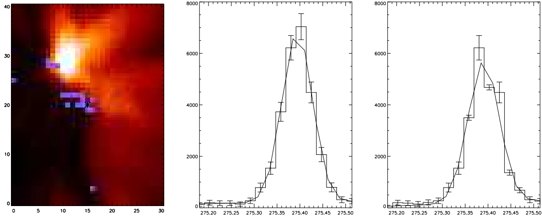
Figure 3: An example of a discrepant pixel for Si VII \lambda 275.35 . The left panel shows an intensity image derived from the original data. The blue pixels denote those for which the intensity derived from data-set processed with the 30 % warm pixel map is more than 1\sigma discrepant from the actual intensity. The pixel for which the line profiles are displayed in the middle and right panels is denoted by a star. The middle panel show the spectrum for the selected spatial pixel from the original data. The right panel shows the spectrum for the data-set processed with the 30 % warm pixel map and for which interpolation over the missing pixels has been performed. For both panels the Gaussian fits to the data are shown over-plotted.
