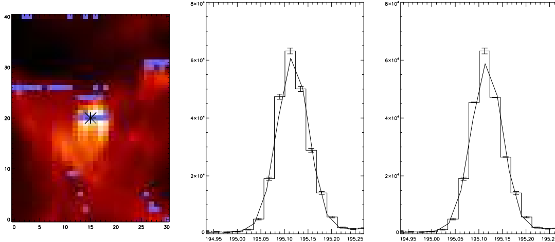
Figure 4: A similar plot to Fig. 3, but for Fe XII \lambda 195.12.
