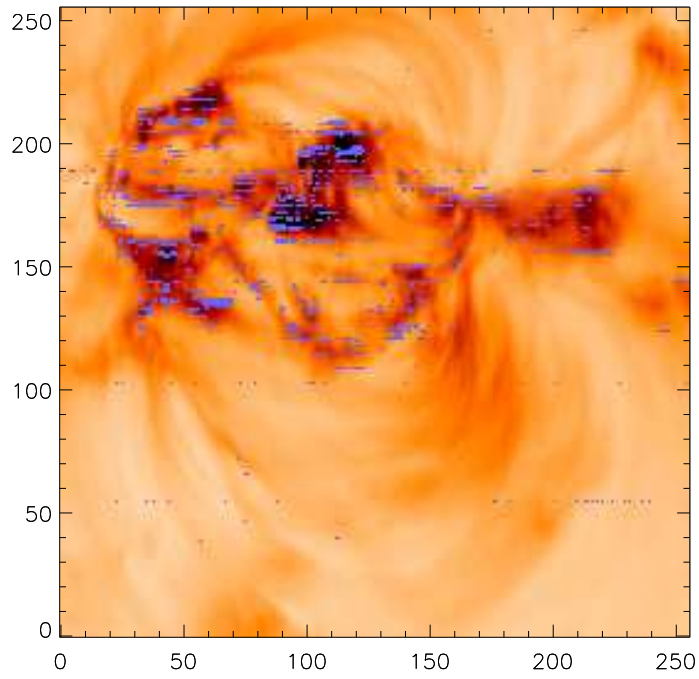
Figure 2: The panels above show negative intensity images from Si VII \lambda 275.35 (upper) and Fe XII \lambda 195.12 (lower) from the 2006 December 2 data-set. Blue pixels denote those spatial pixels that fail the conditions given in Eqs. 3 and 4.
