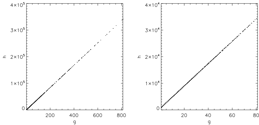
Figure 1: Plots of h vs. g for a sub-set of full CCD data from 2007 January 30 14:34 UT. The left panel shows the full range of the data values, the right panel shows the same data but with the g range reduced by a factor 10.
