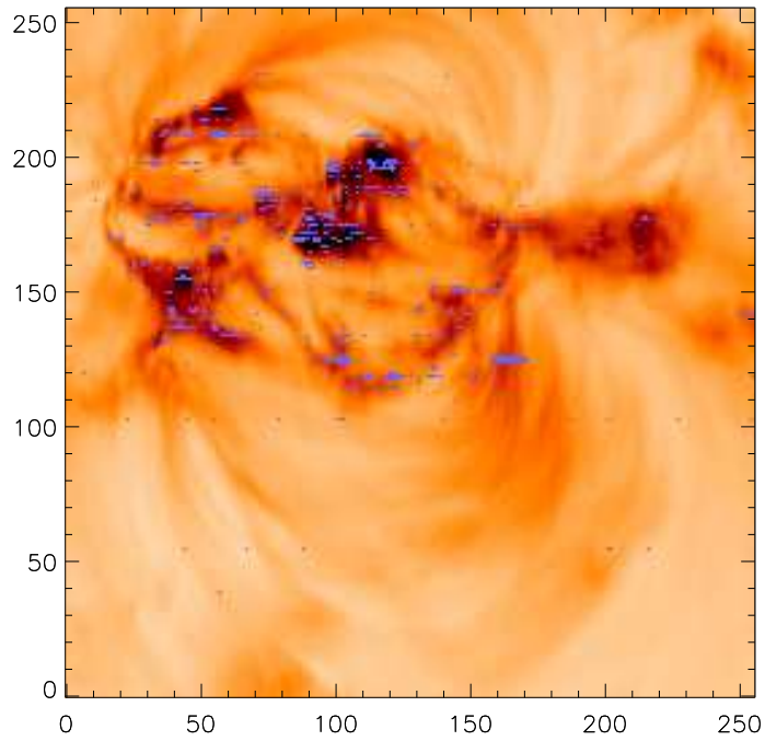
Figure 5: The panels above show negative intensity images from Si VII \lambda 275.35 (upper) and Fe XII \lambda 195.12 (lower) from the 2006 December 2 data-set. Blue pixels denote those spatial pixels that fail the conditions given in Eqs. 3 and 4.
