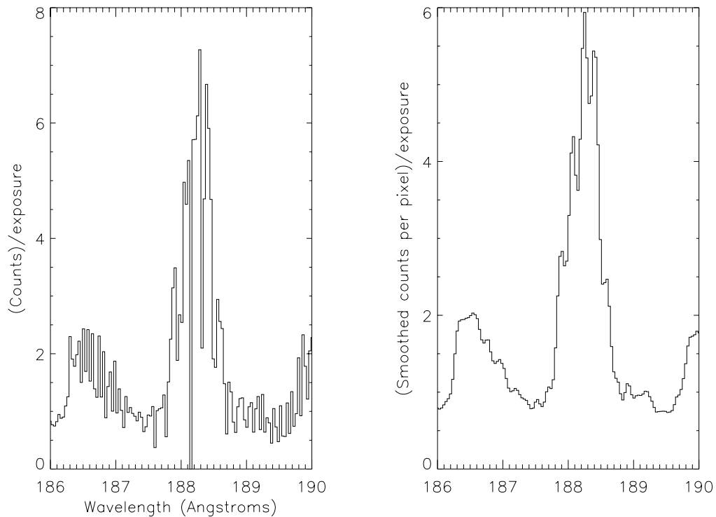
Figure 1: A plot of the data around an Fe XI line from study 10716, showing fixed patterning (left plot), where data shows large variations from pixel to pixel . The right plot shows the same data after running gis_smooth .
